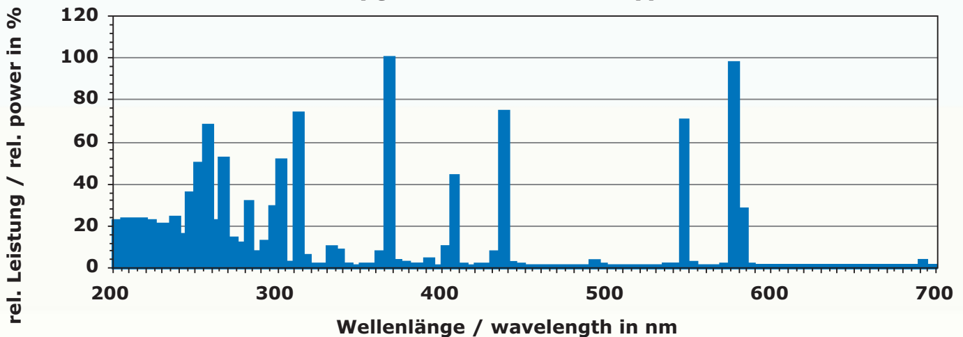
Spektrum UVH-Strahler, Typ Standard / Spectrum UVH-lamp, type standard (Quecksilber / Mercury)
