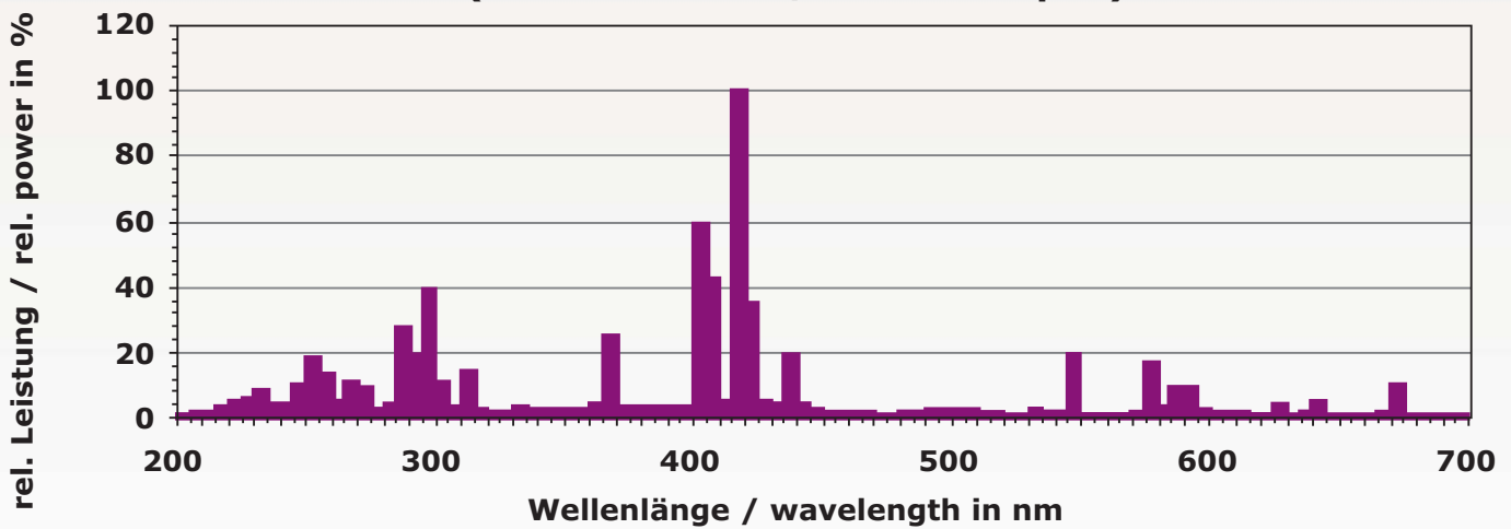
Spektrum UVH-Strahler, Typ Ga / Spectrum UVH-lamp, type Ga (Gallium dotiert / Gallium doped)
